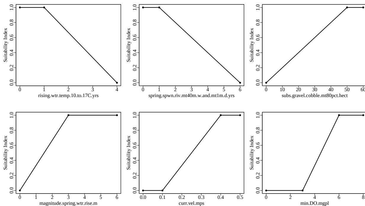
Figure 1. Suitability index graphs for variables included in the paddlefishSpwnHab model in ecorest .
