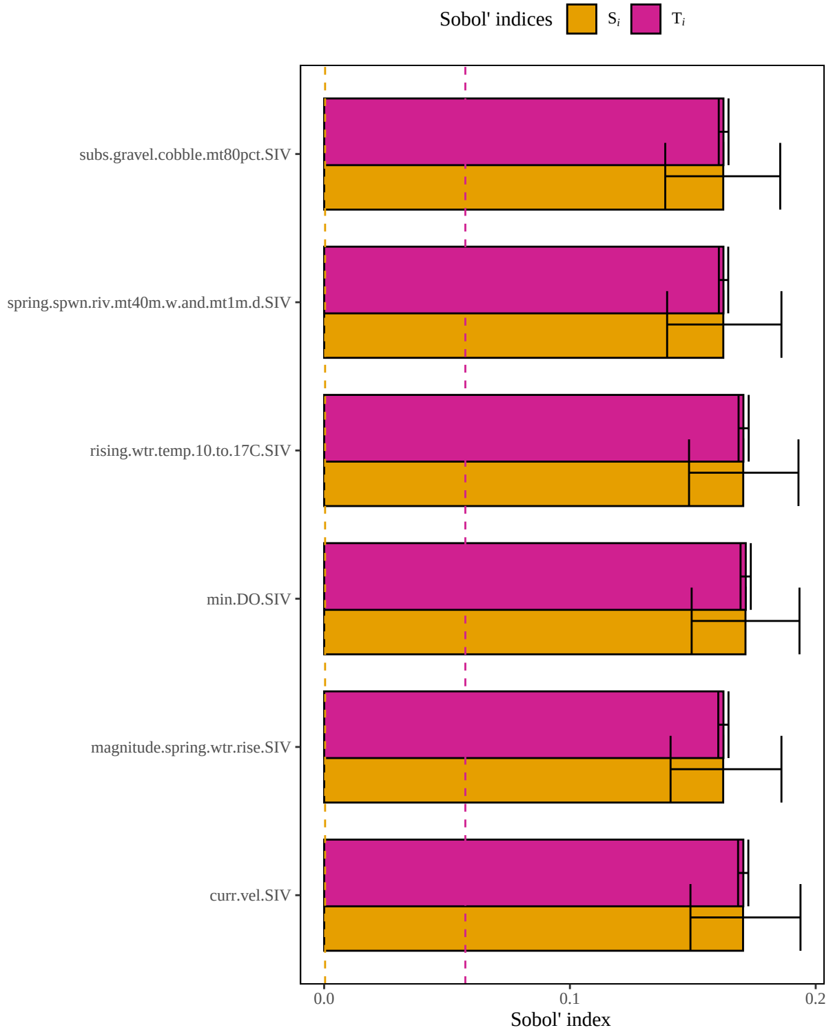
Figure 4. Results of a sensitivity analysis for the paddfishSpwnHab model based on an arithmetic mean structure. Dashed lines represent baseline numerical approximation error for S_i and T_i ( i.e. , dummy variables).
