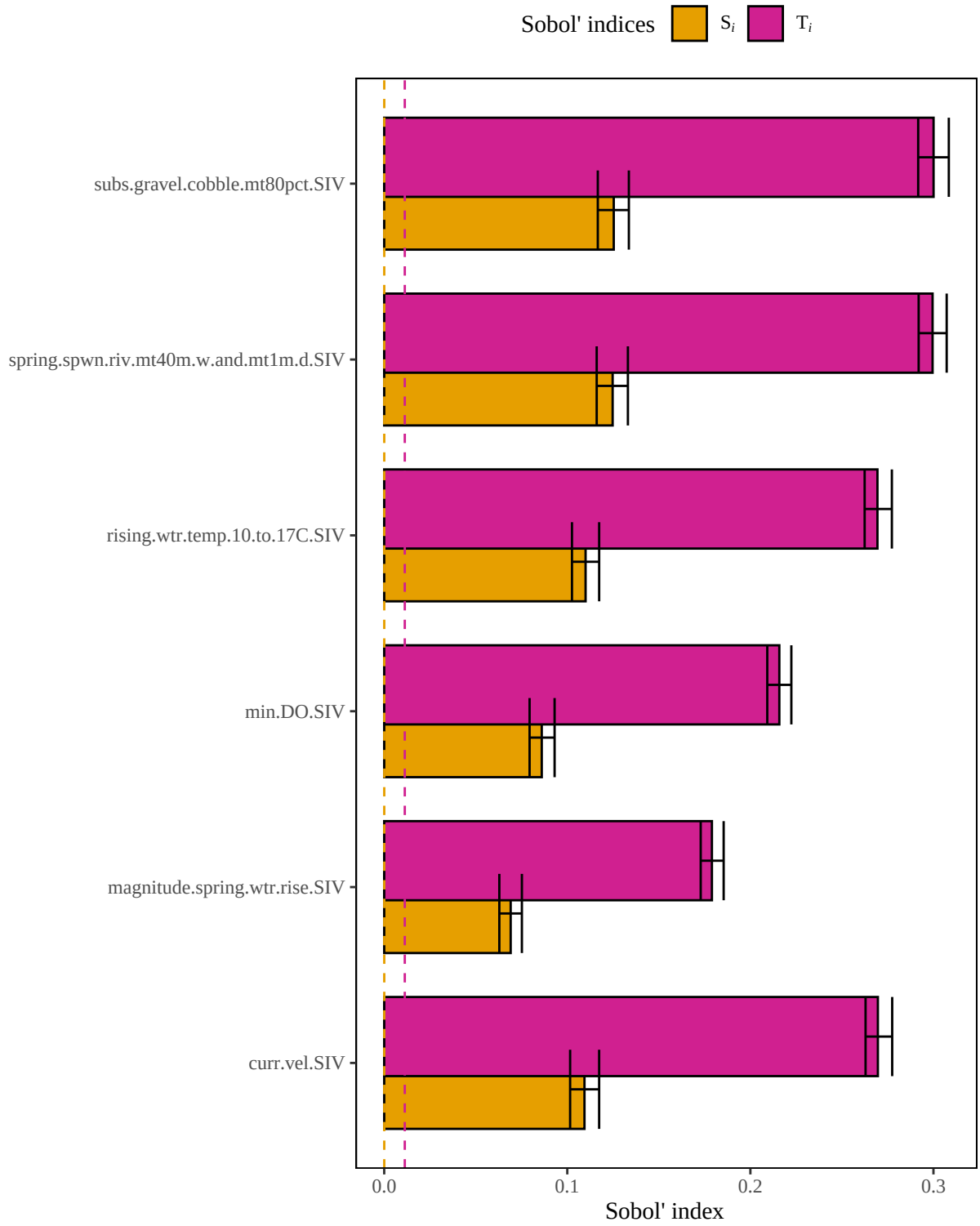
Figure 6. Results of a sensitivity analysis for the paddlefishSpwnHab model based on a limiting factor structure. Dashed lines represent baseline numerical approximation error for S_i and T_i ( i.e. , dummy variables).
