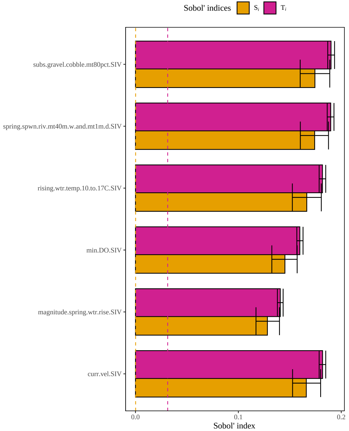
Figure 5. Results of a sensitivity analysis for the paddfishSpwnHab model based on a geometric mean structure. Dashed lines represent baseline numerical approximation error for S_i and T_i ( i.e. , dummy variables).
