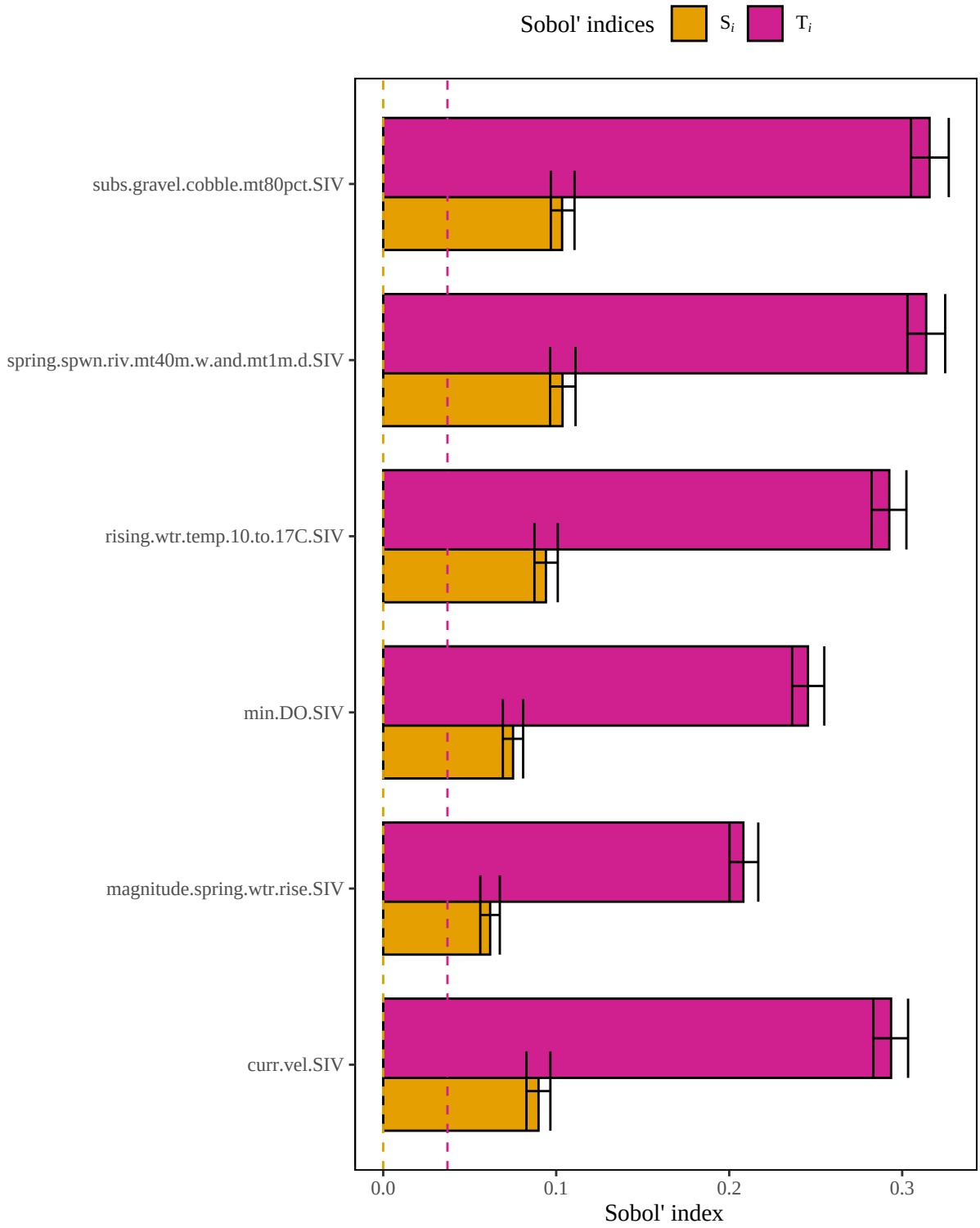
Figure 7. Results of a sensitivity analysis for the paddfishSpwnHab model based on a multiplicative mean structure. Dashed lines represent baseline numerical approximation error for S_i and T_i ( i.e. , dummy variables).
